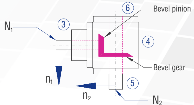
Figure 5.3.3-1; Shaft designations
