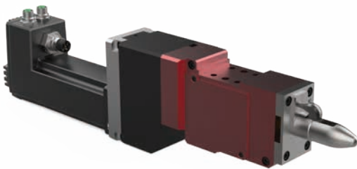
92P Electric Centering Pin Clamp
